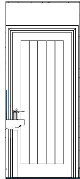
A WC - View A 1 : 25
