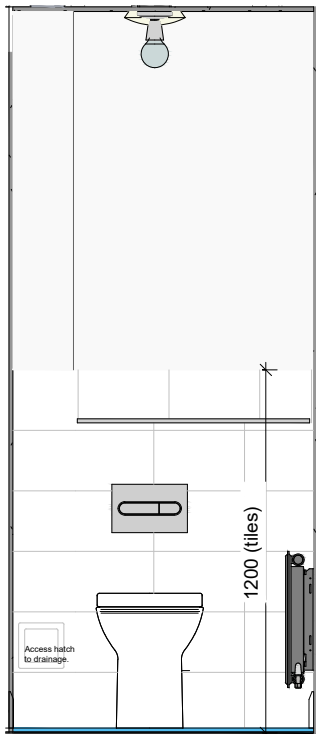
C WC - View C 1 : 25
