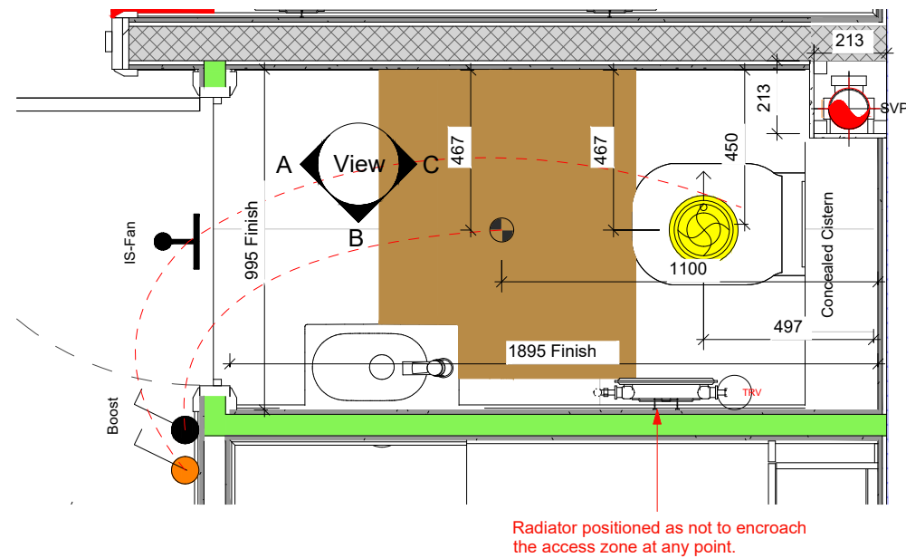
1 Ground Floor W/C Layout 1 : 20
