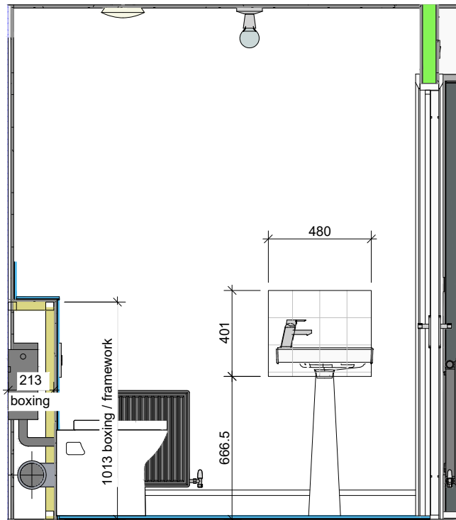
B WC - View B 1 : 25
